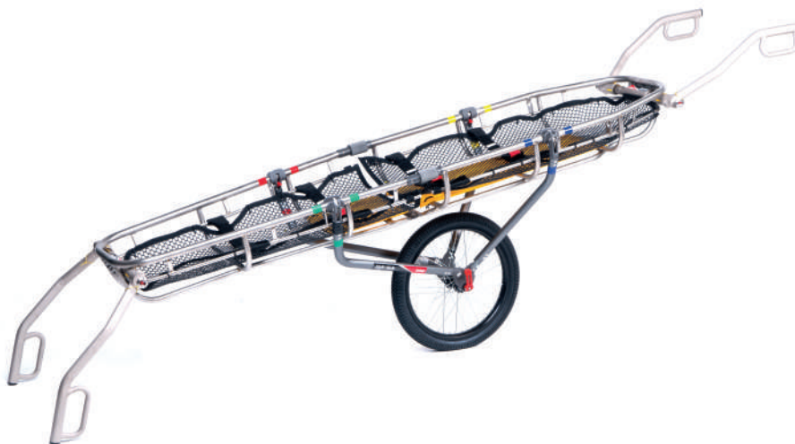
TIROL KIT FOT TITAN-TI BASKET STRETCHER WITH WELDED PLATES
